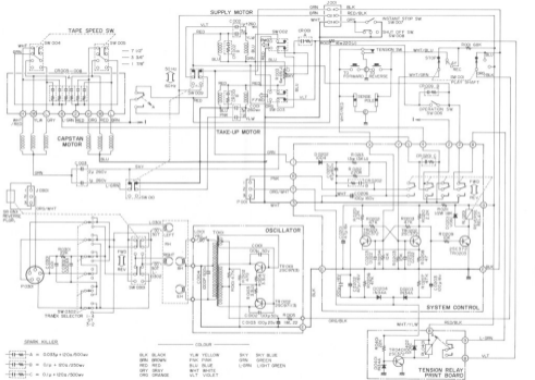
M-I-O MECHANISM SCHEMATIC DIAGRAM NO.2-1 I381654I
